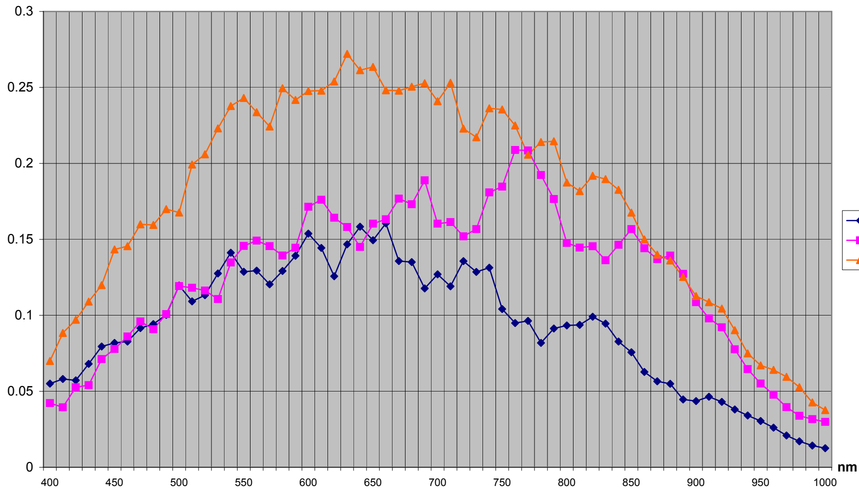
Spectral Response IBIS 1300 sensors
