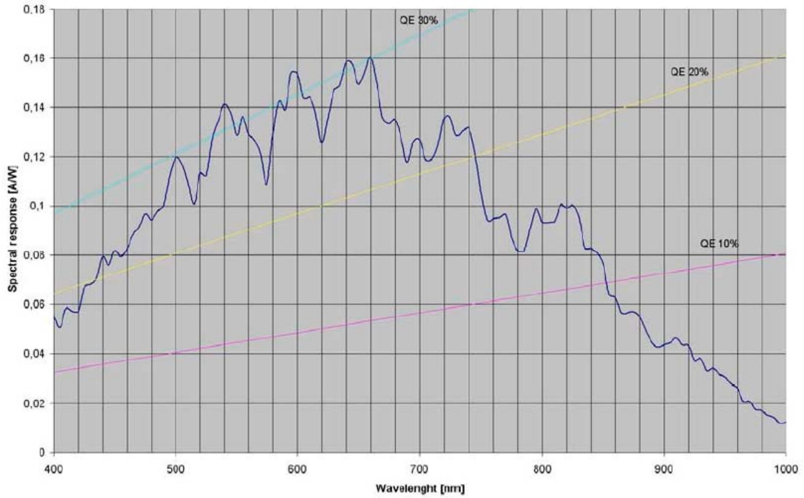
IBIS5 Spectral Response Curve
