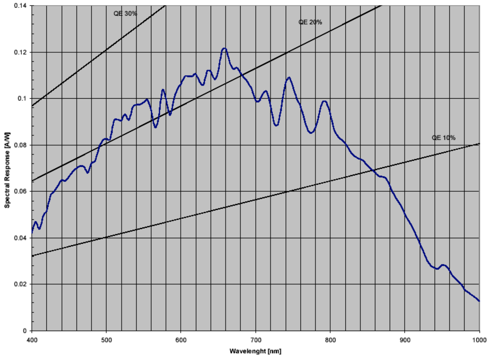
IBIS4-6600 Spectral Response Curve
