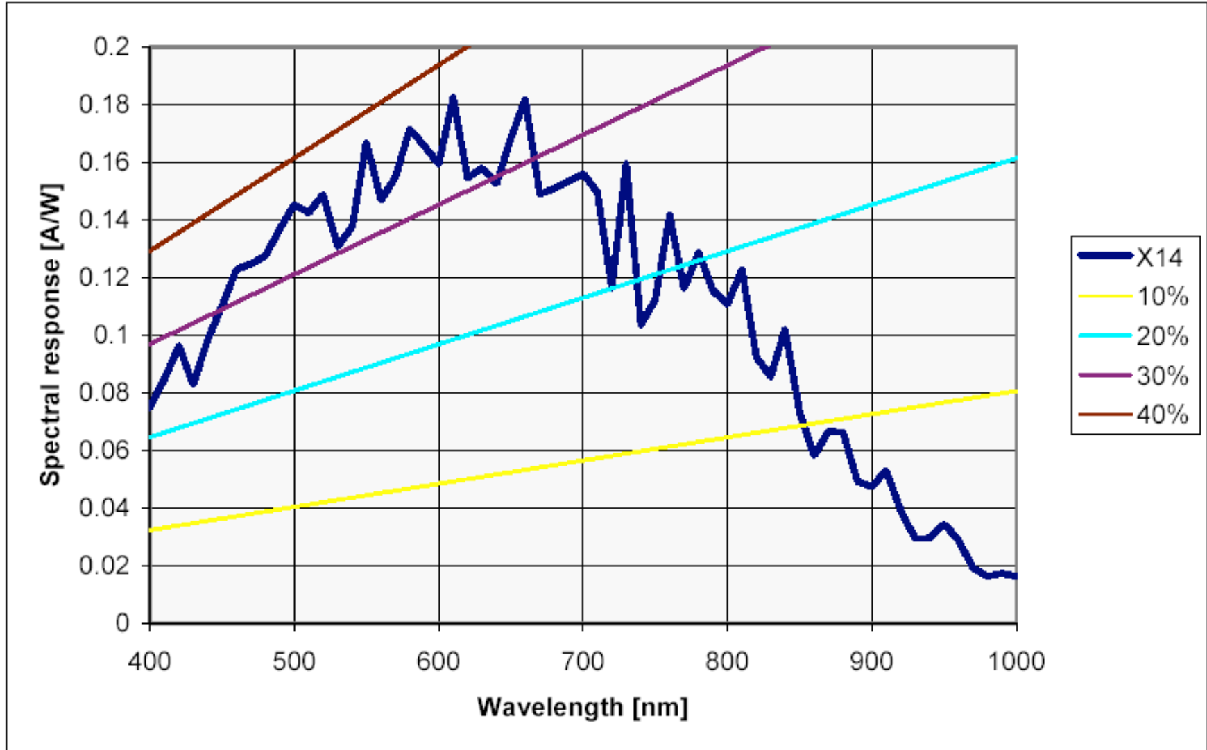
IBIS4-14000 Response Curve
